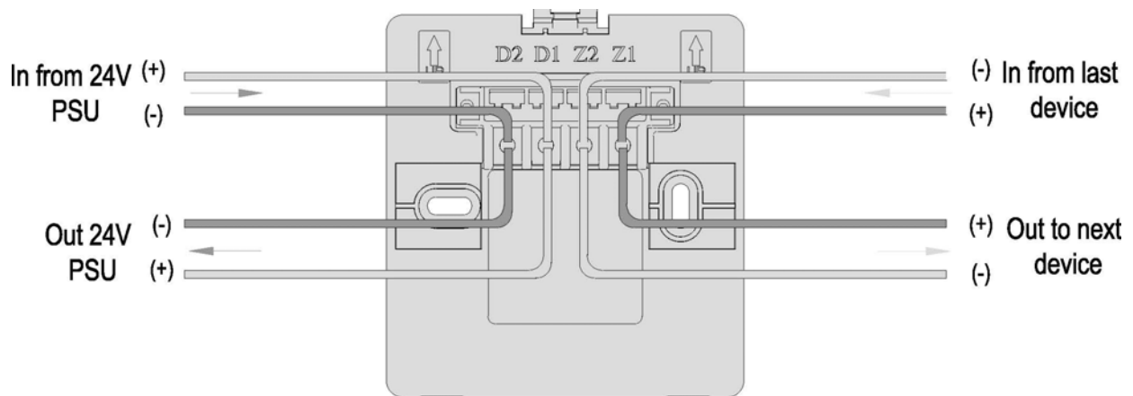
Figure 3: Wiring Details
